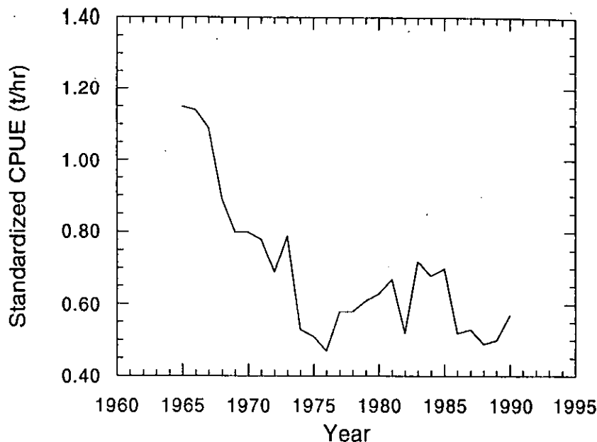
Fig. 29. Yellowtail flounder in Div. 3LNO: standardized catch rates.
