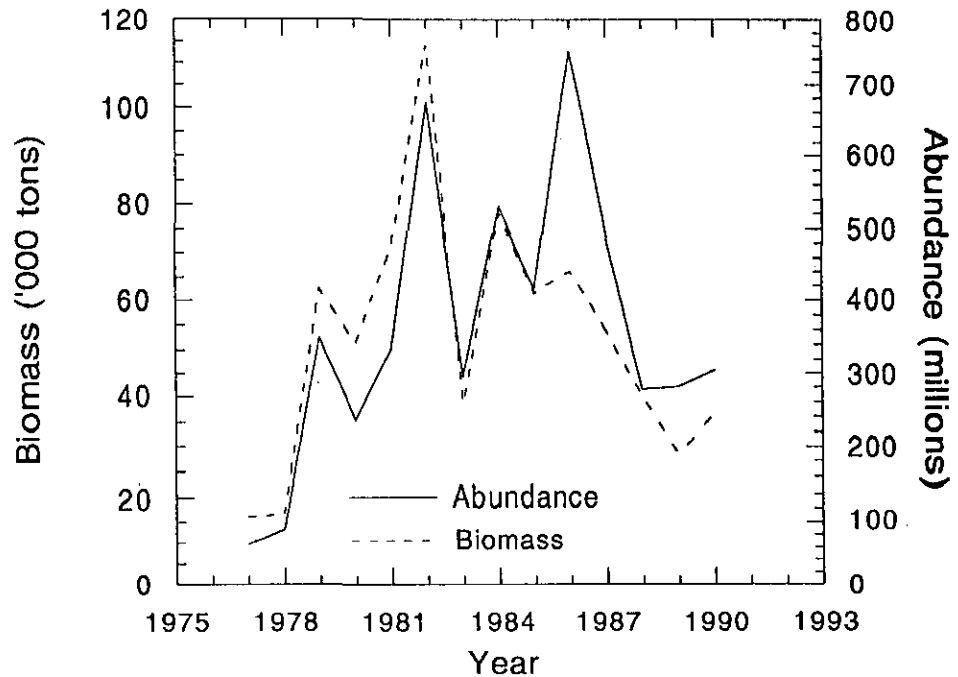
Fig. 20. Silver hake in Div. 4VWX: biomass and abundance estimates from July Canadian research vessel data.
