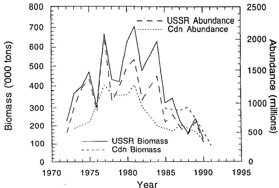
Fig. 25. American plaice in Div. 3LNO: biomass and abundance estimates from research vessel data.
