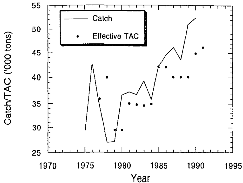
Fig. 39. Shrimp in Subareas 0 and 1: catches and TACs in offshore Subarea 1 (south of 71°N) and adjacent areas in Subarea 0 (Div. 0A). Effective TACs from 1977 to 1980 for Subarea 1 only.
