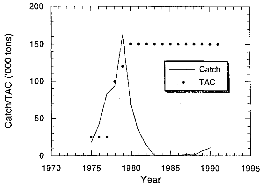
Fig. 38. Squid in Subareas 3 and 4: catches and TACs.
