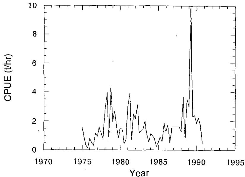
Fig. 4. Cod in Subarea 1: CPUE by quarter for six sister trawlers owned by the Greenland Home Rule.
