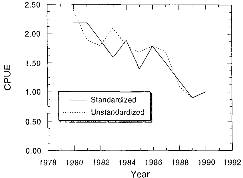
Fig. 42. Shrimp in Denmark Strait: catch rates.
