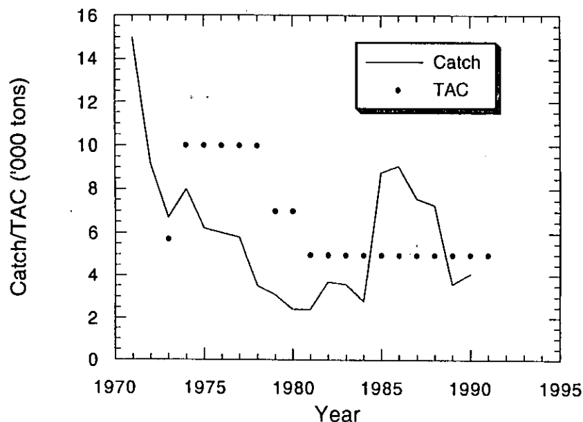
Fig. 26. Witch flounder in Div. 3NO: catches and TACs.
