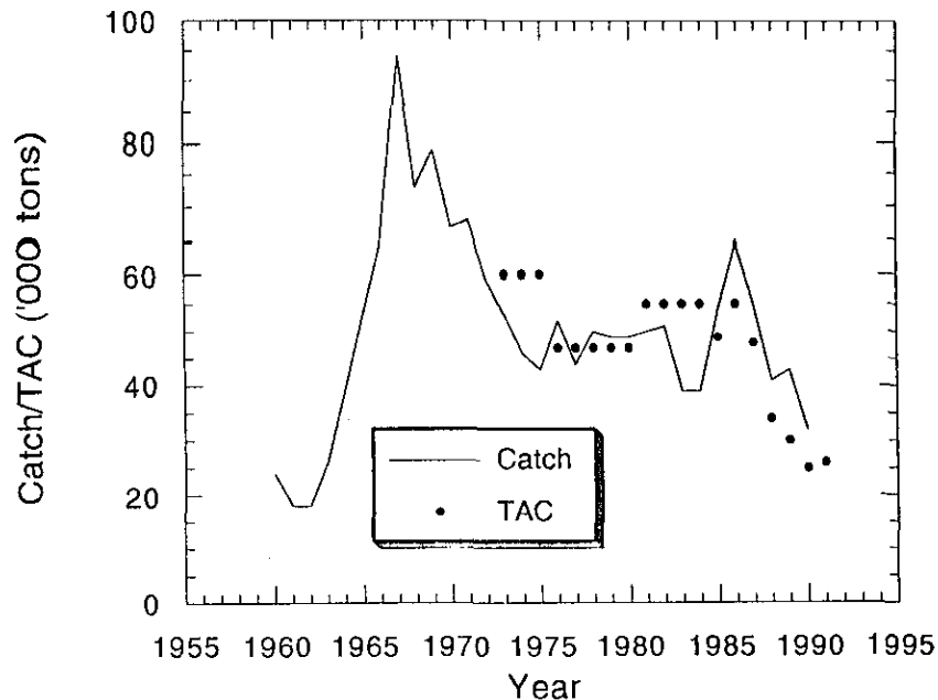
Fig. 23. American plaice in Div. 3LNO: catches and TACs.
