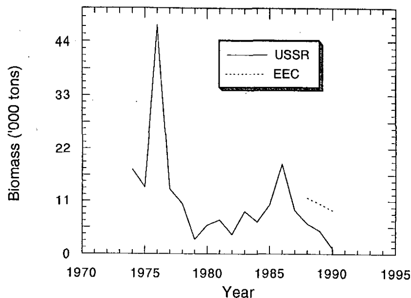
Fig. 22. American plaice in Div. 3M: biomass estimates from research vessel data.
