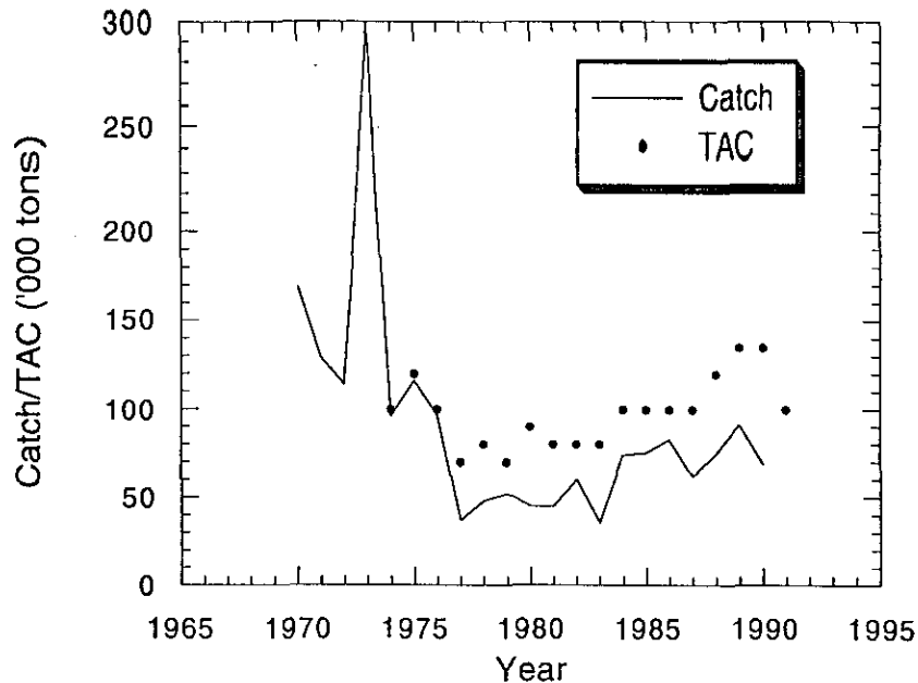
Fig. 18. Silver hake in Div. 4VWX: catches and TACs.
