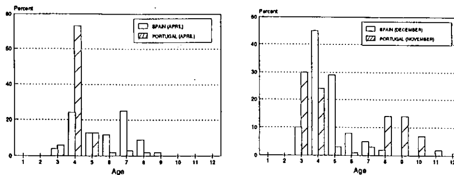
Fig. 2. Cod in Div. 2J and 3KL: spring and autumn catch-at-age for EEC-Spain and EEC-Portugal fisheries.
