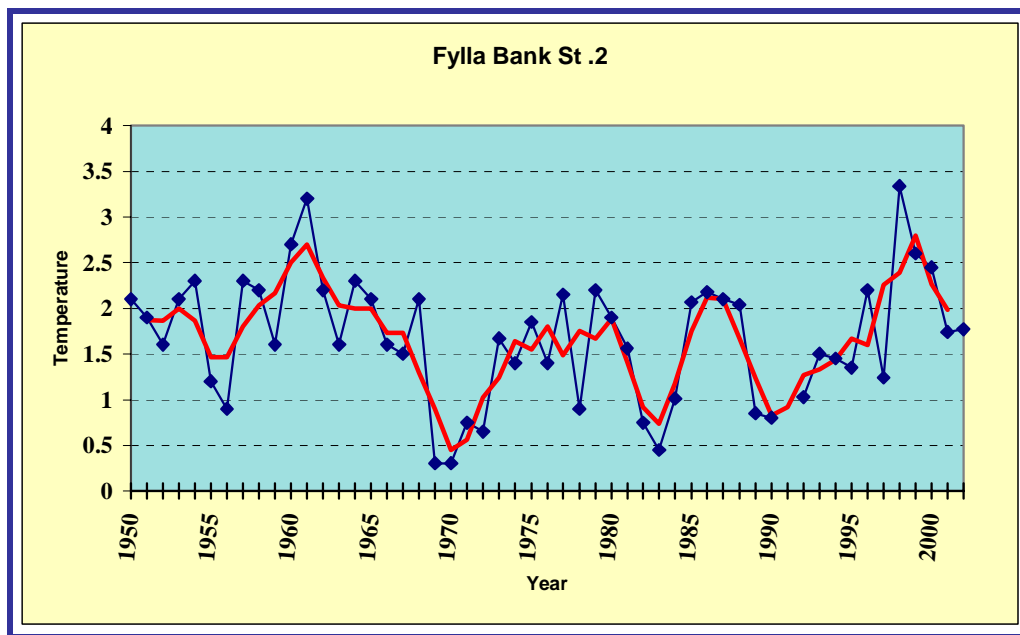
Fig. 4. Time series of mean temperature (observations and 3-year running mean) on top of Fylla Bank (0 - 40 m) in the middle of June.
