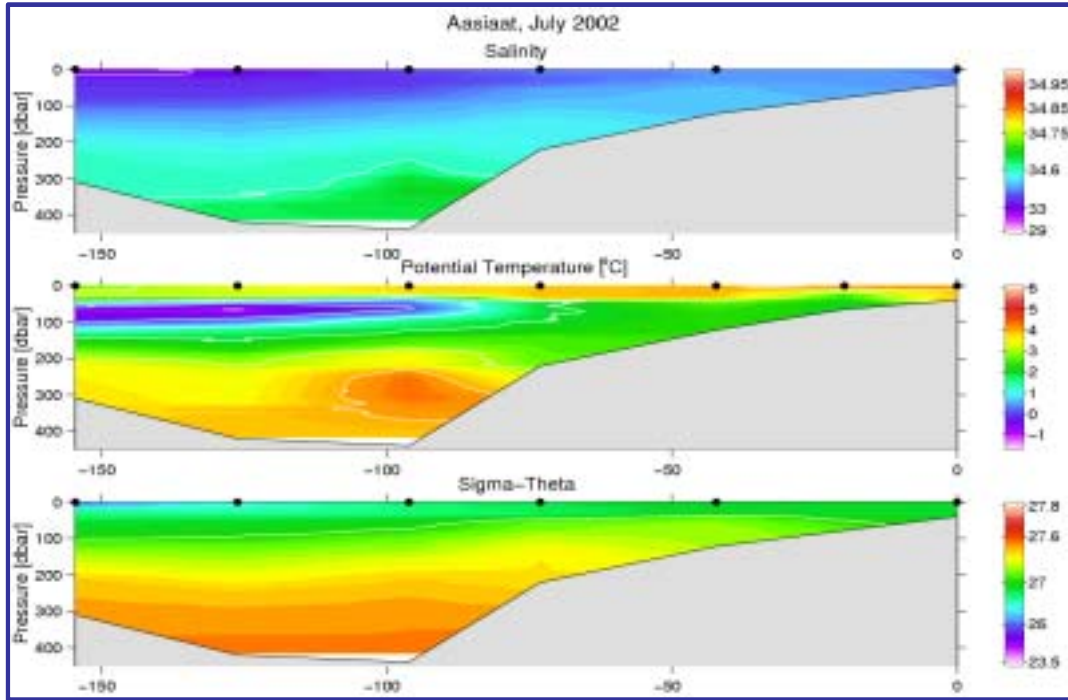
Fig. 15. Vertical distribution of temperature, salinity and density at the Aasiat Section, July, 2002.
