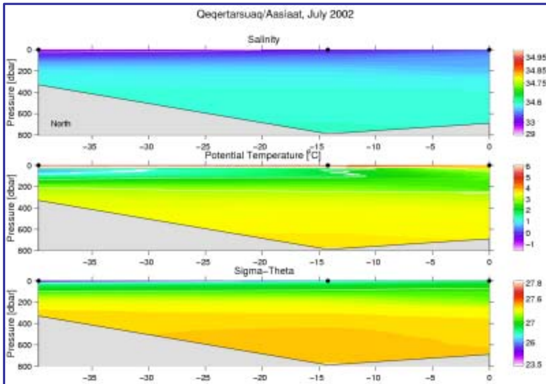
Fig. 16. Vertical distribution of temperature, salinity and density at the Qeqertarsuaq.Aasiat Section, July 2002.
