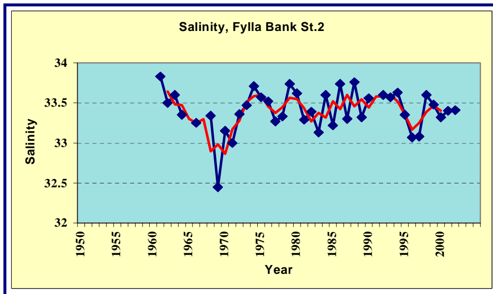
Fig. 8. Time-series of the mean salinity (observations and 3-year running mean) on top Fylla Bank (0-40 m) in the middle of June.
