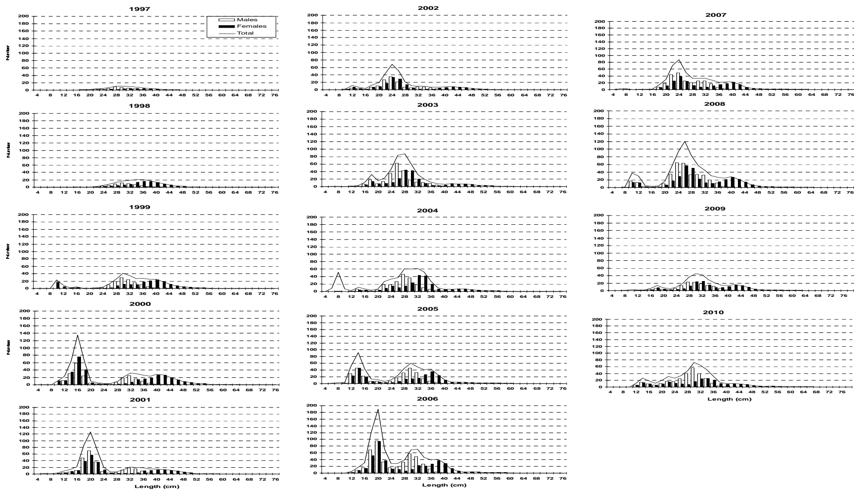
FIGURE 10.- American plaice length distribution (cm) on NAFO 3NO: 1997-2010. Estimated numbers per haul stratified mean catches. 1997-2000 data are transformed data from C/V Playa de Menguña , and 2002-2010 data are original from R/V Vizconde de Eza . In 2001, there are data from the two vessels.
