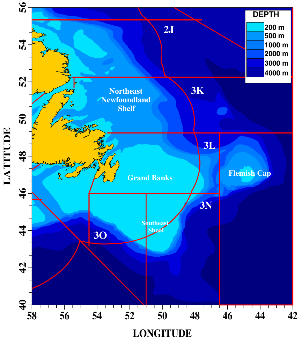
Figure 1. NAFO areas of interest for the assessment of Newfoundland Ecoregions (2J3KLNO). The major bathymetric zones showing the Northeast Newfoundland Shelf, Grand Banks, Flemish Cap as well as the Southeast Shoal region at the tail of the Grand Banks.
